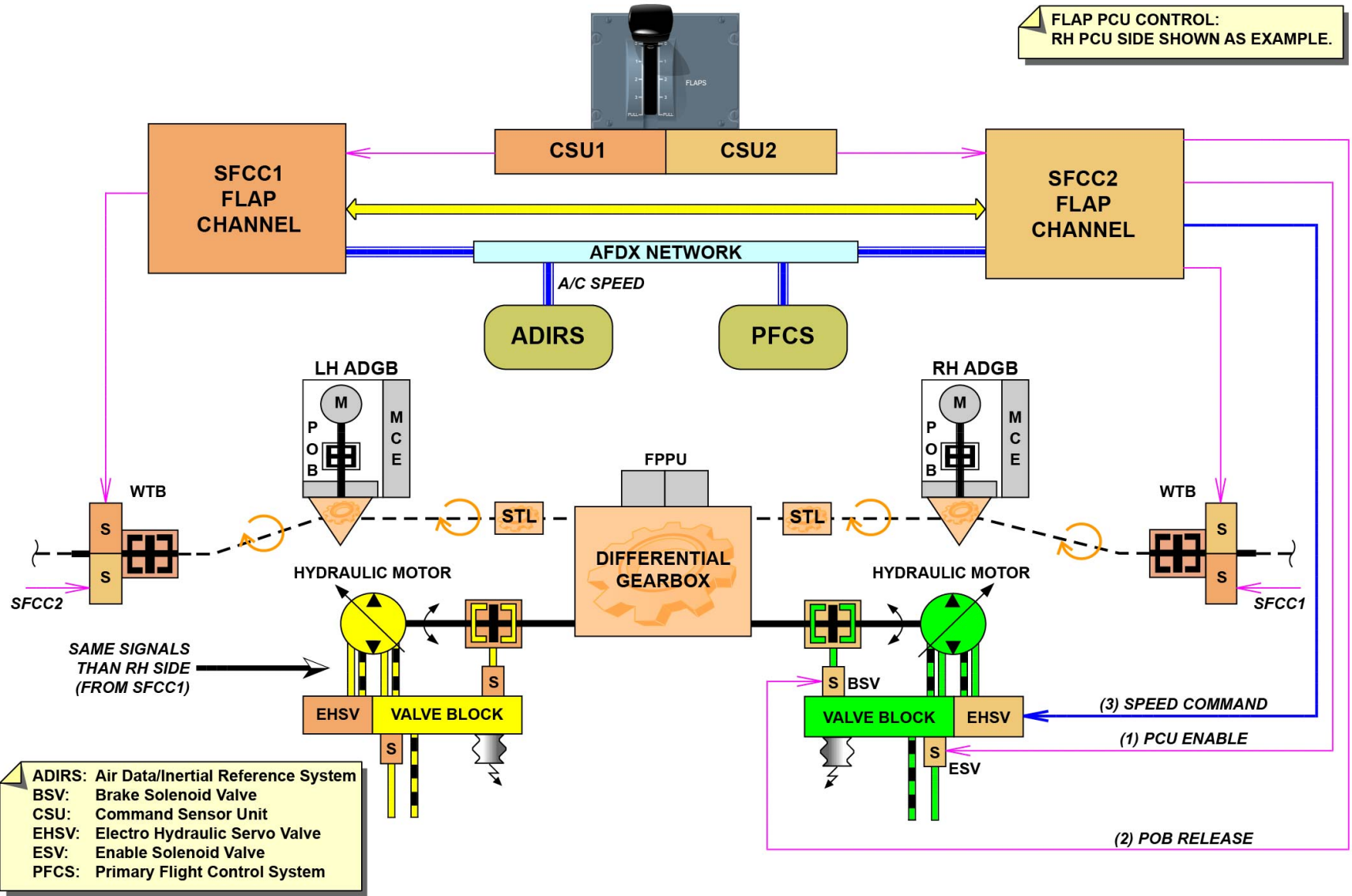
COMPUTATION GROUP - FLAP SYSTEM CONTROL
