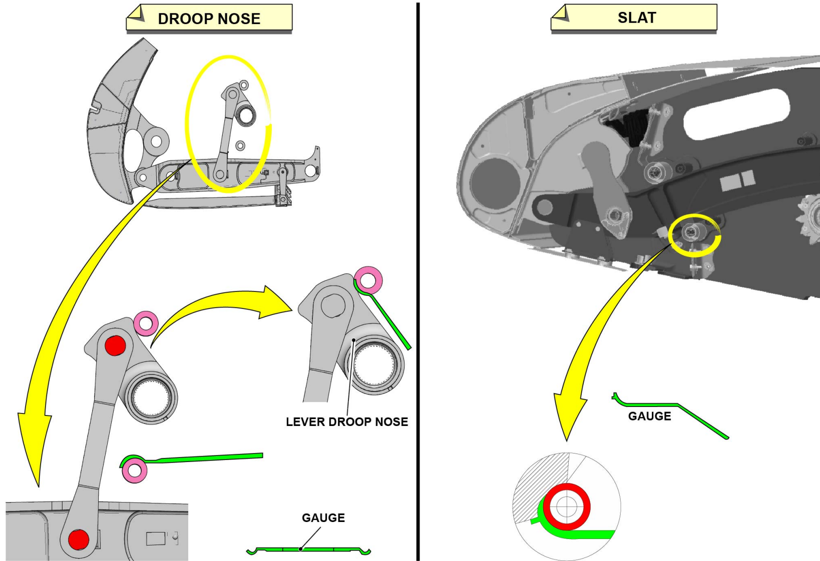
SLAT FLAP RIGGING PROCEDURE
