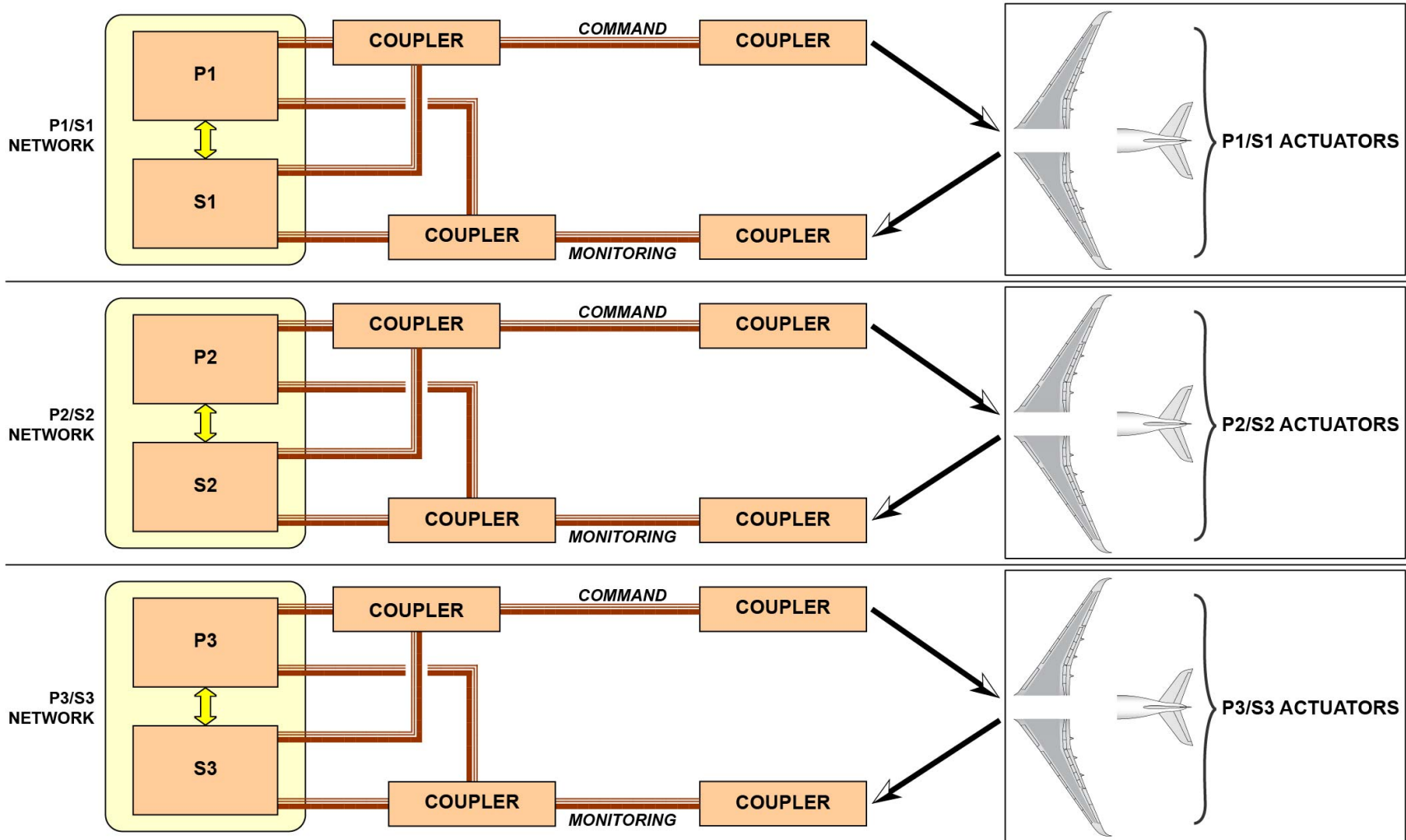
FLIGHT CONTROL ARCHITECTURE
