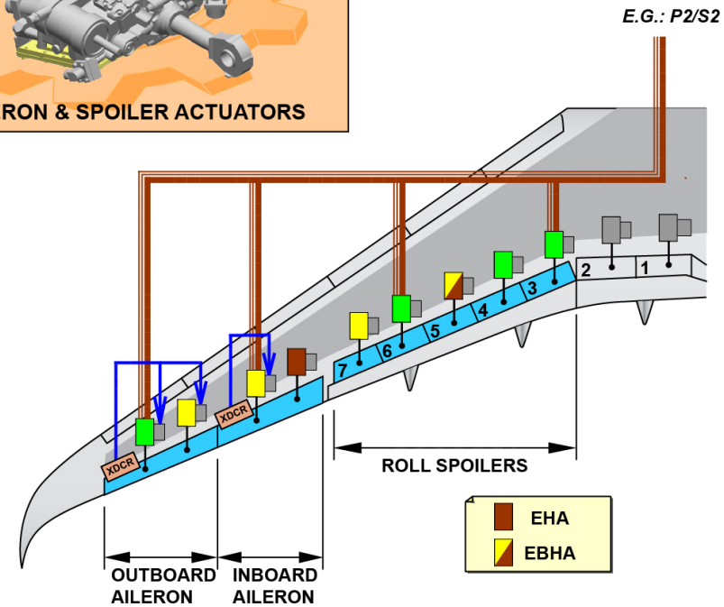
LATERAL FUNCTION: ROLL DESCRIPTION
