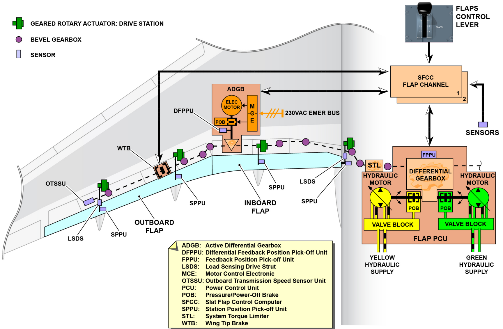
COMPUTATION GROUP - FLAP SYSTEM DESCRIPTION
