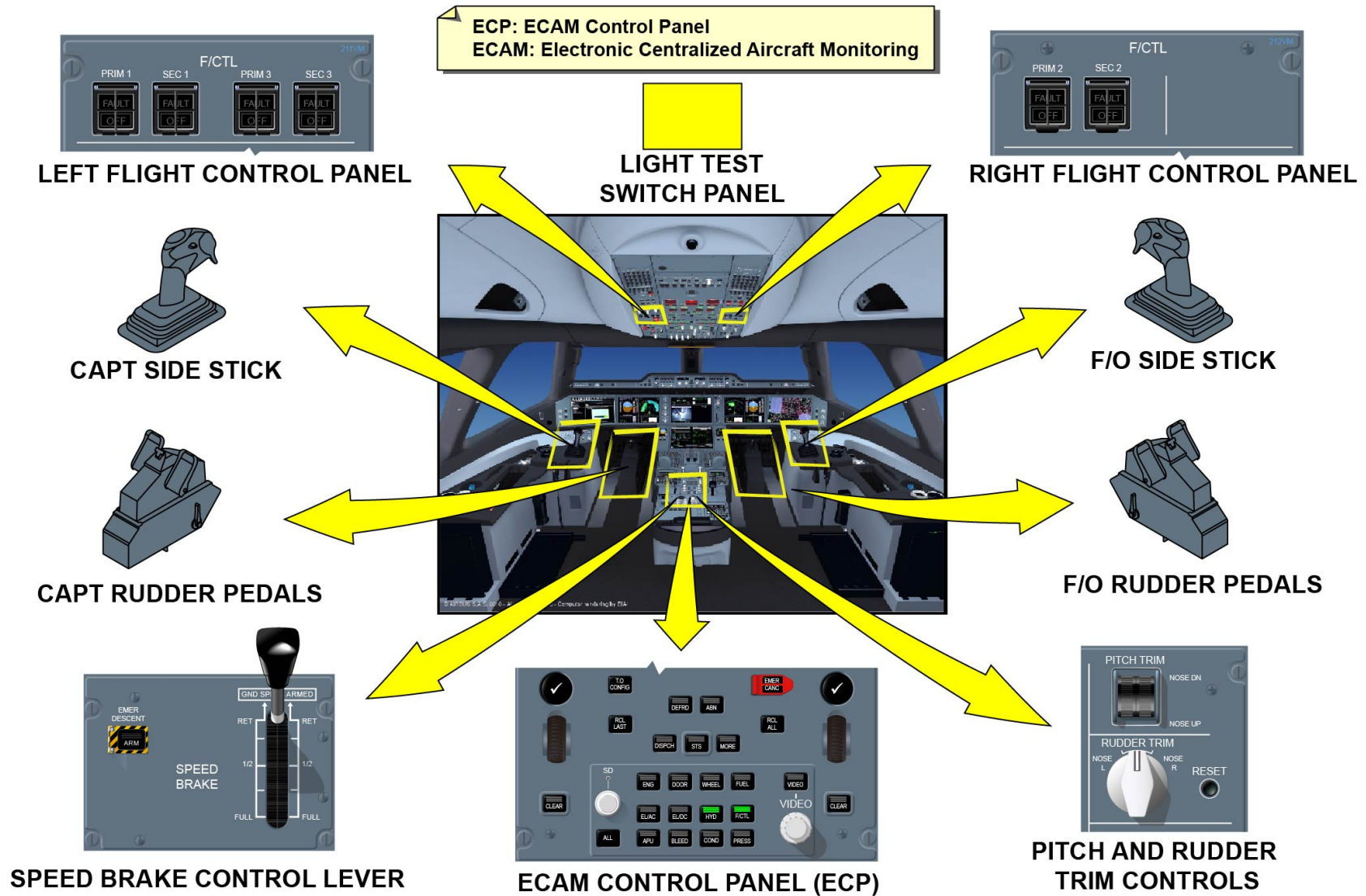
PRIMARY FLIGHT CONTROL - GENERAL (2) ... RUDDER CONTROL FAILURE (3)
