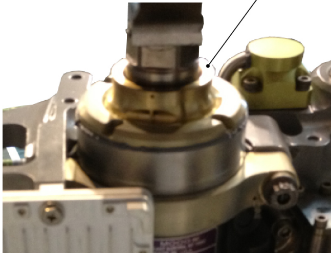
SERVOCONTROL BEFORE COLLAR INSTALLATION
