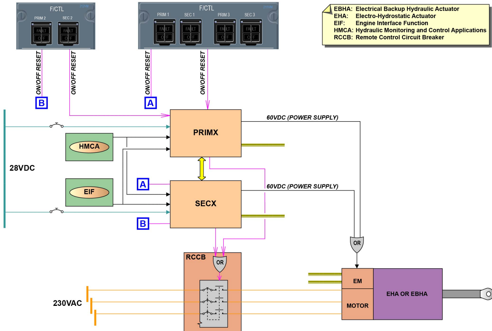
POWER SUPPLY: COMPUTER, ACTUATOR AND FCRM/ELECTRONIC MODULES
