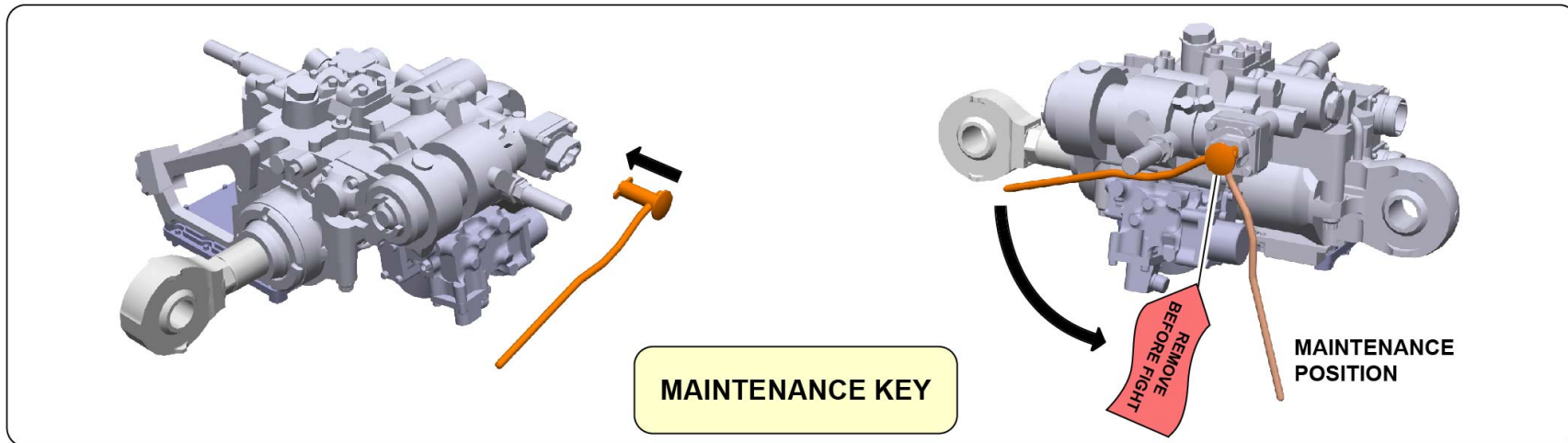
SPOILER SERVO-CONTROL COMPONENTS
