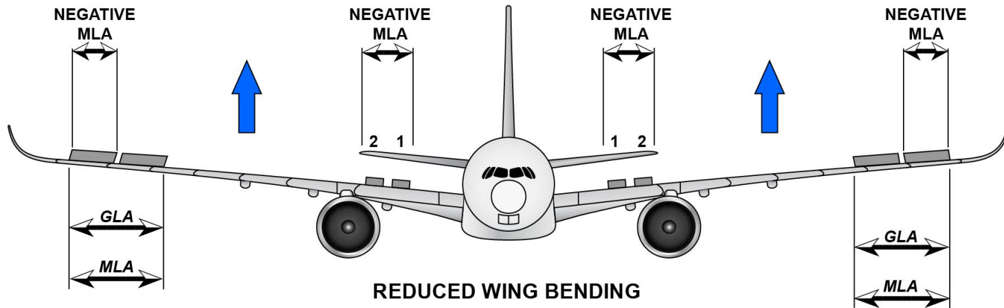
LOAD ALLEVIATION FUNCTION
