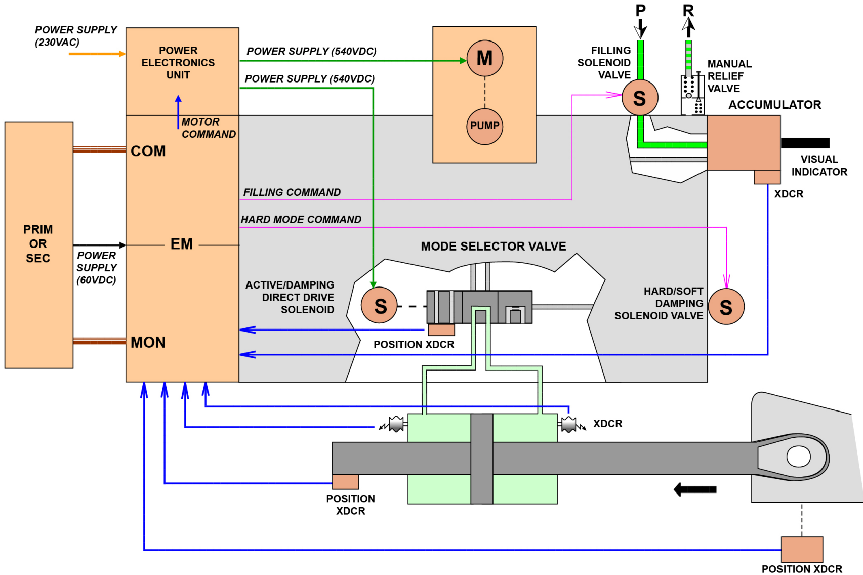
ACTUATORS GROUP: EHA PRINCIPLE
