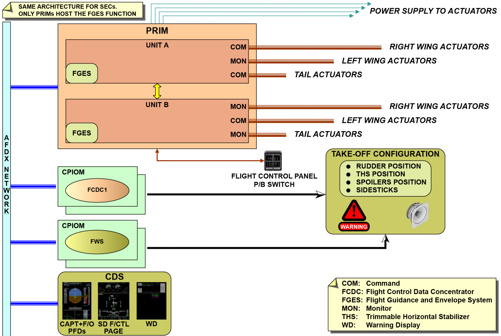
PRIMS, SECS AND FCDCS
