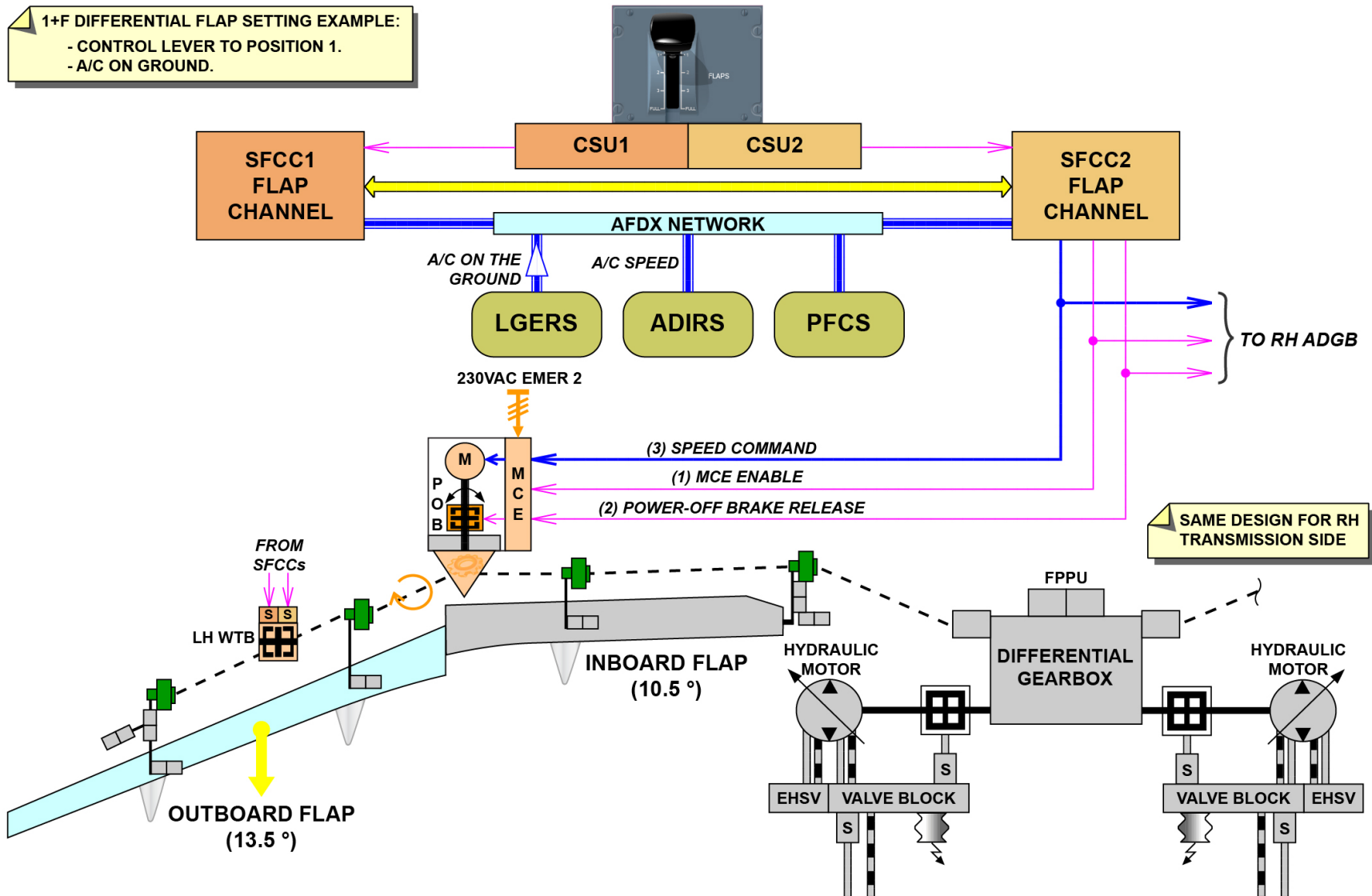
COMPUTATION GROUP - ADGB CONTROL: DIFFERENTIAL FLAP SETTING INTRODUCTION
