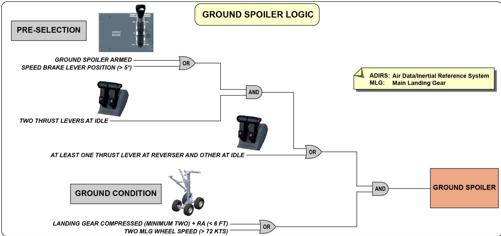
GROUND SPOILER ACTUATION
