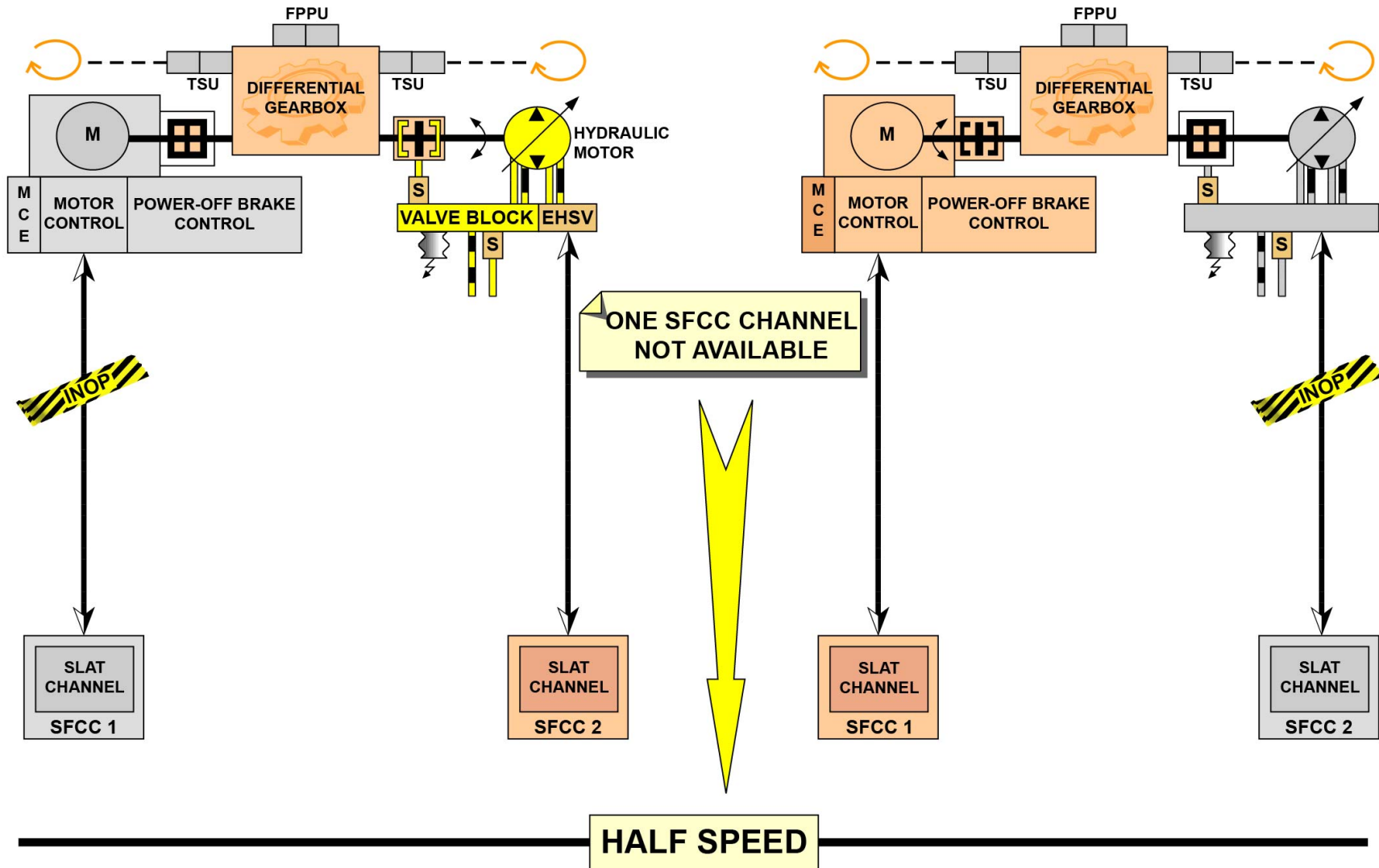
SLAT SYSTEM HALF-SPEED CONFIGURATION
