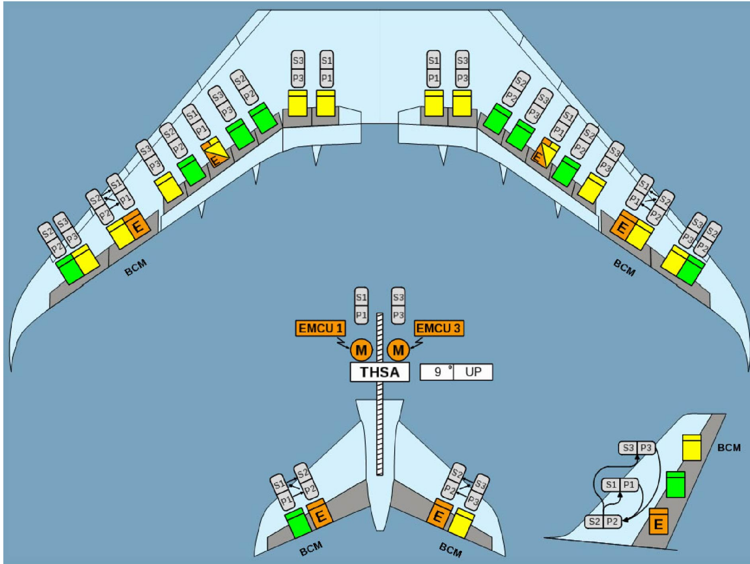
PRIMARY FLIGHT CONTROL - GENERAL (2) ... RUDDER CONTROL FAILURE (3)
