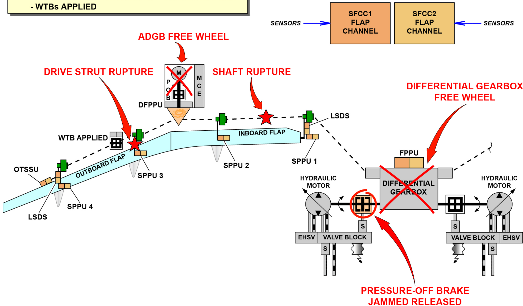
TRANSMISSION AND ACTUATION GROUP FAILURES - MECHANICAL FAILURES
