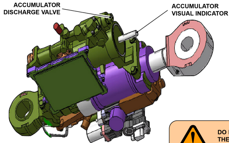
ACCUMULATOR DISCHARGE VALVE
