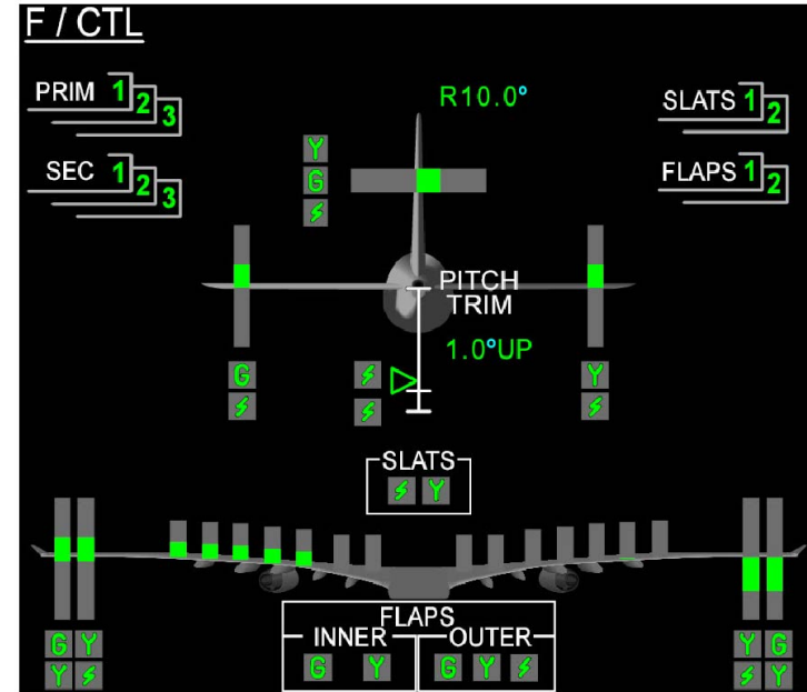
SD FLIGHT CONTROL PAGE
