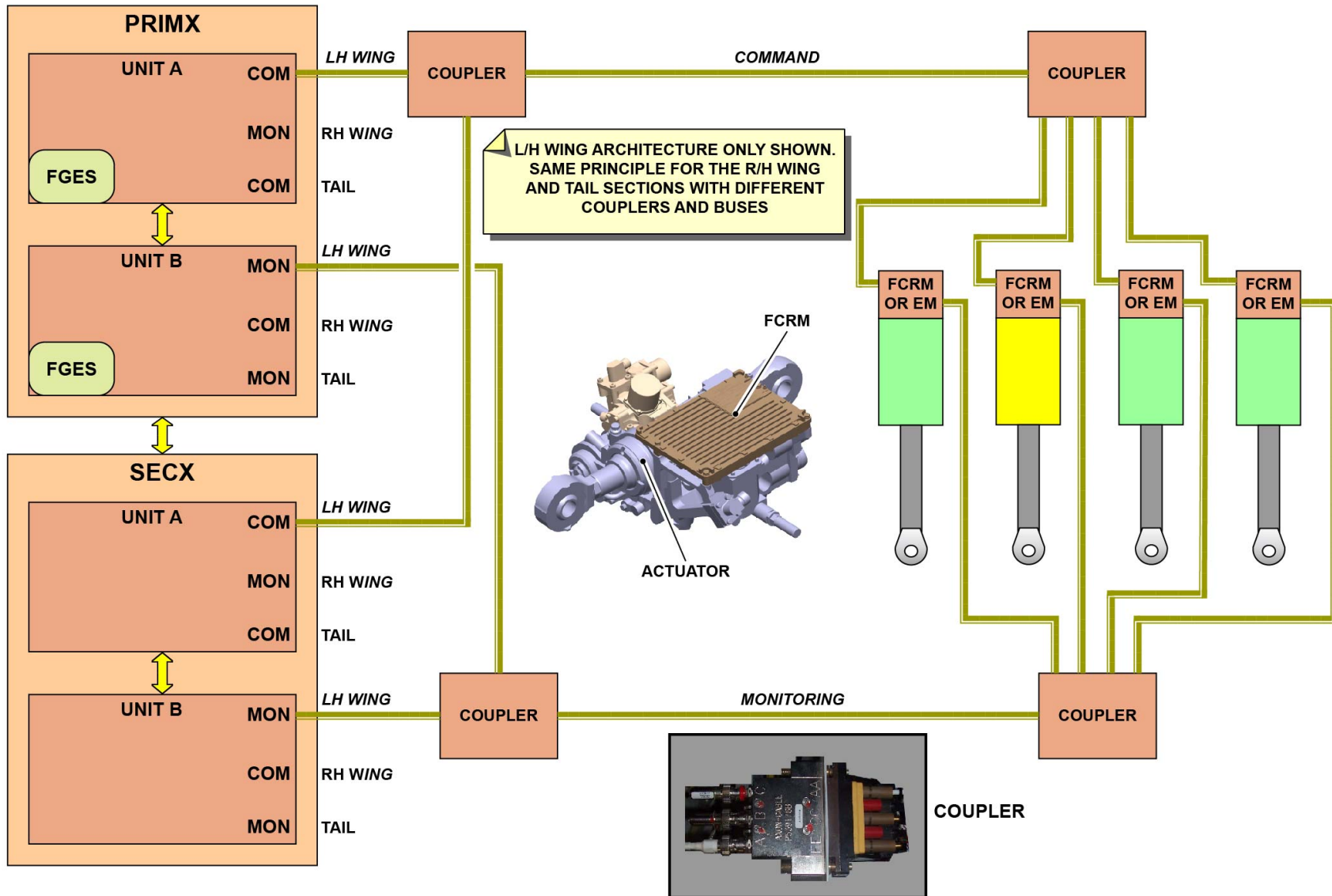
MIL 1553 FLIGHT CONTROL ARCHITECTURE
