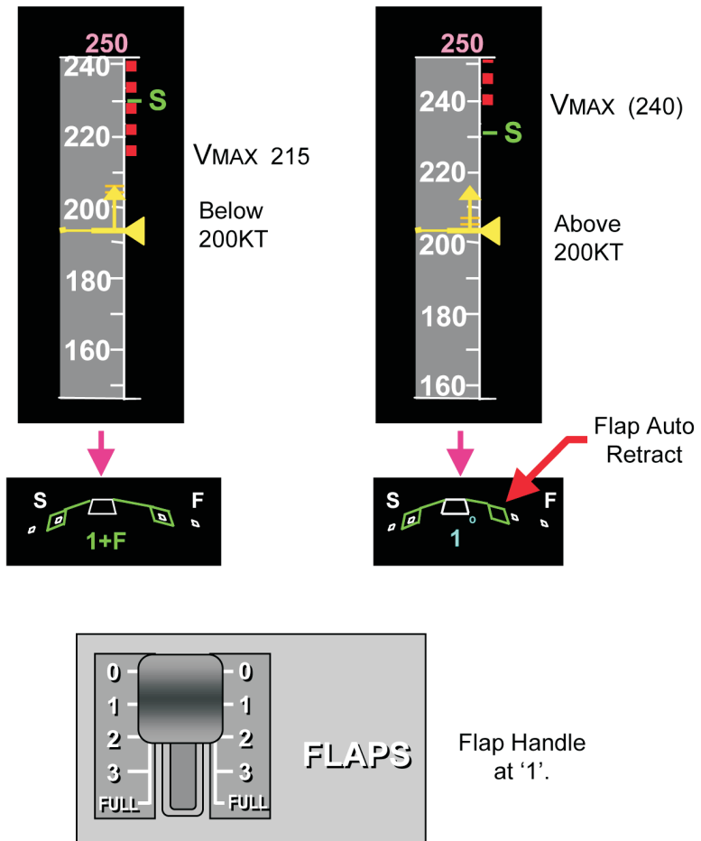
Flaps Auto Retraction Indications (Example for A333)
