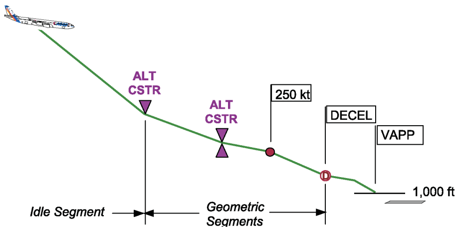
FMGS Descent Profile
