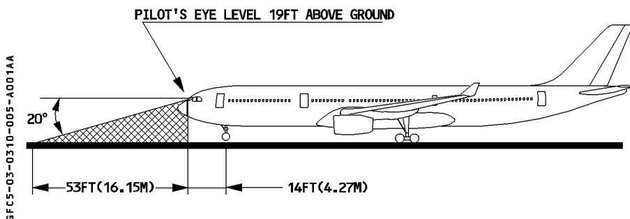
Visual Ground Geometry
